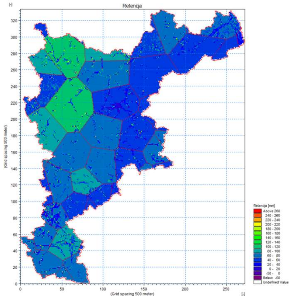
Figure 1: Calculation results: map of 1-day retention totals in the Pilica catchment area
