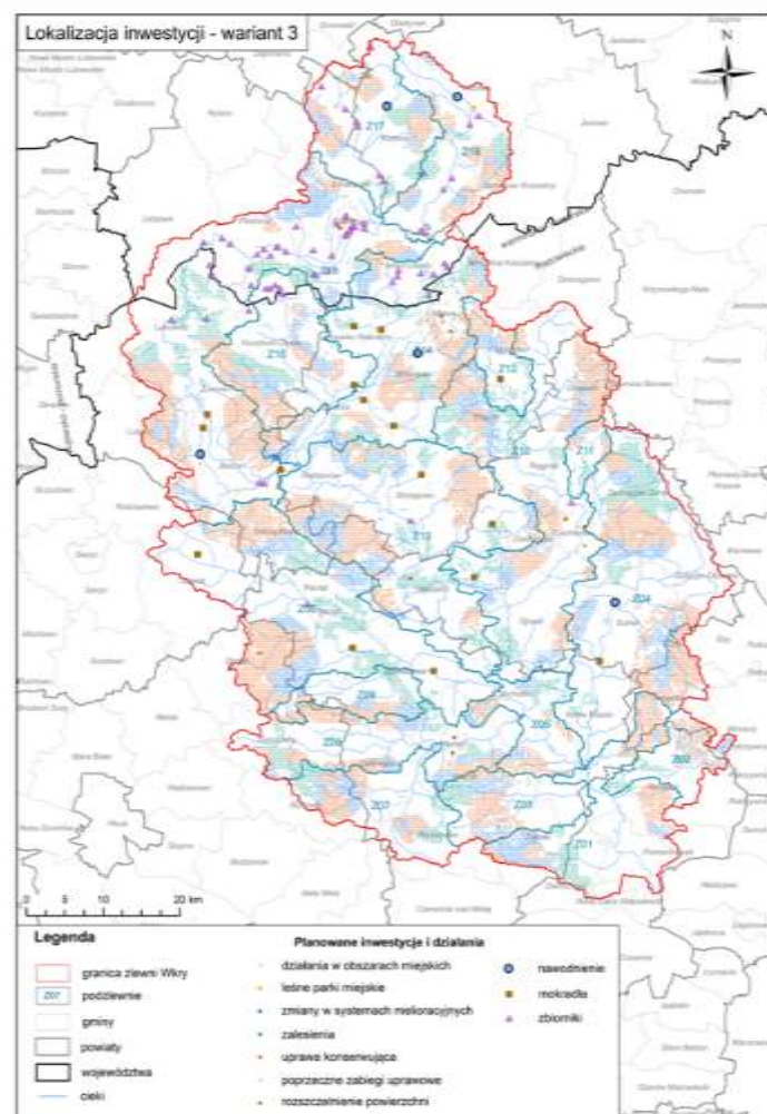
Figure 3: Location of activities and tasks from variant 3 increasing retention for the Wkra catchment area.
