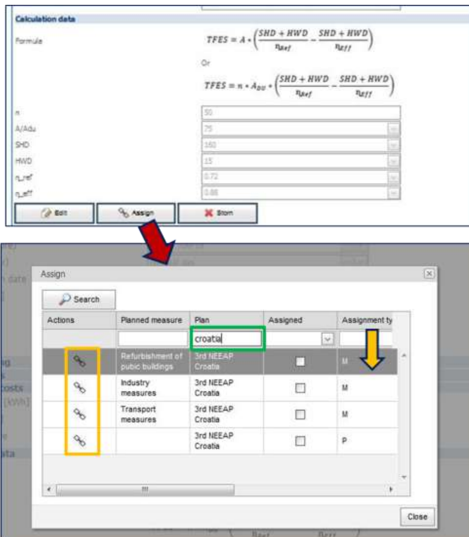
Figure 27: Part of the implemented measure (top) and assignment window (bottom).
